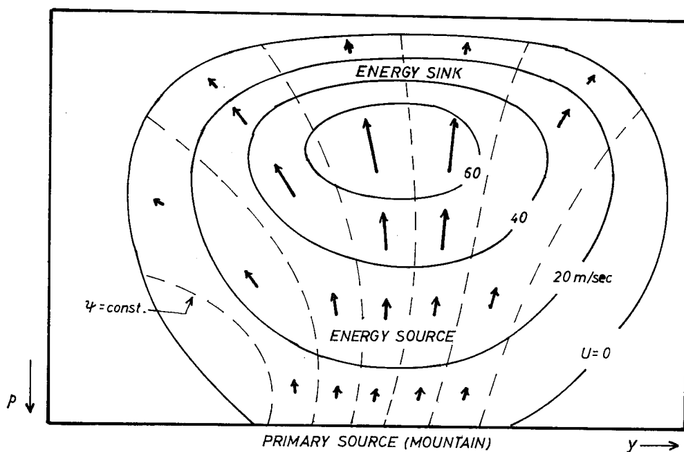
Fig. 6. Meridional flow of wave energy. Solid lines: isotachs of zonal wind. Dashed lines: Wave energy streamlines. Arrows indicate wave energy flux.
